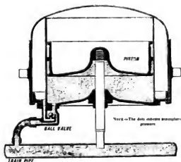
Fig. 5128. Brakes Applied.
